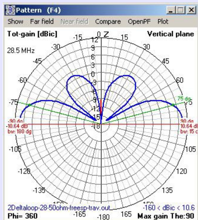
Fig 7 DL-Special DX 0.25 \lambda above the ground
