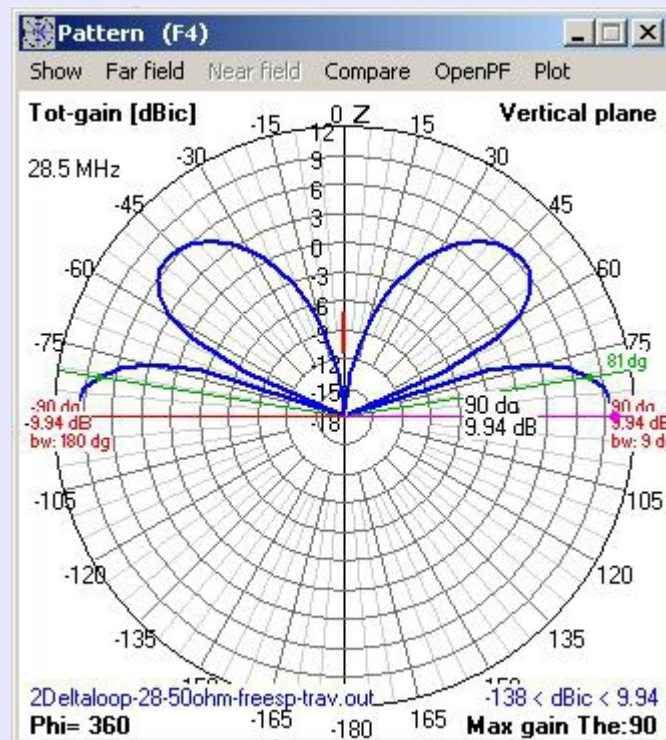
Fig 9 DL-Special DX 0.5 \lambda above the ground
