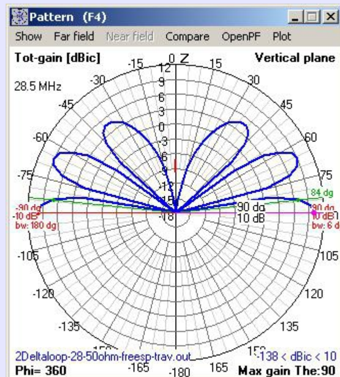
Fig 10 DL-Special DX 1 \lambda above the ground
